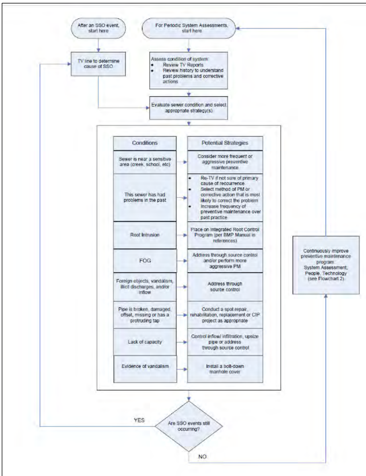
Figure 4-4 SSO Prevention Flowchart
