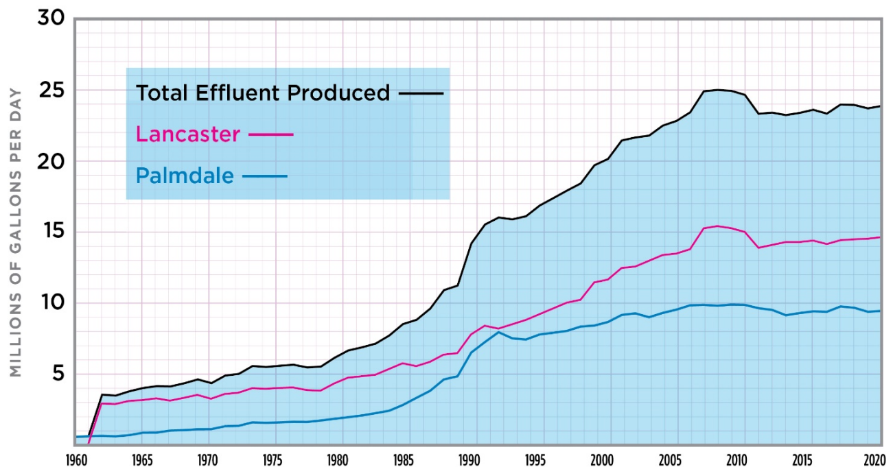
FIGURE 17 ANTELOPE VALLEY WRPs INFLUENT FLOW 1960-2019
