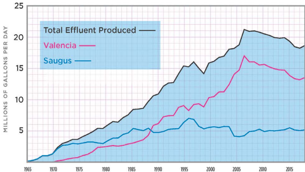
FIGURE 15 SANTA CLARITA VALLEY JOINT SEWERAGE SYSTEM RECYCLED WATER PRODUCTION 1962-2017
