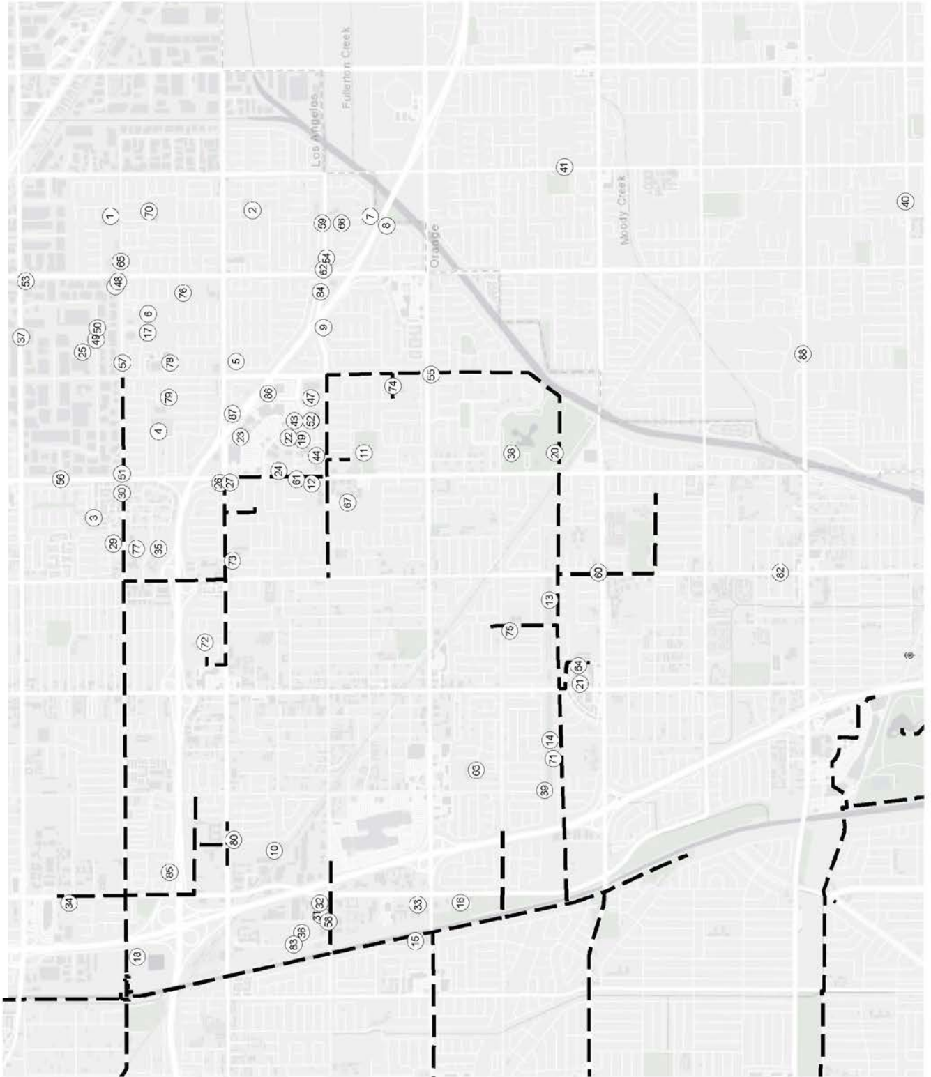
FIGURE 8 CITY OF CERRITOS RECYCLED WATER DISTRIBUTION SYSTEM
