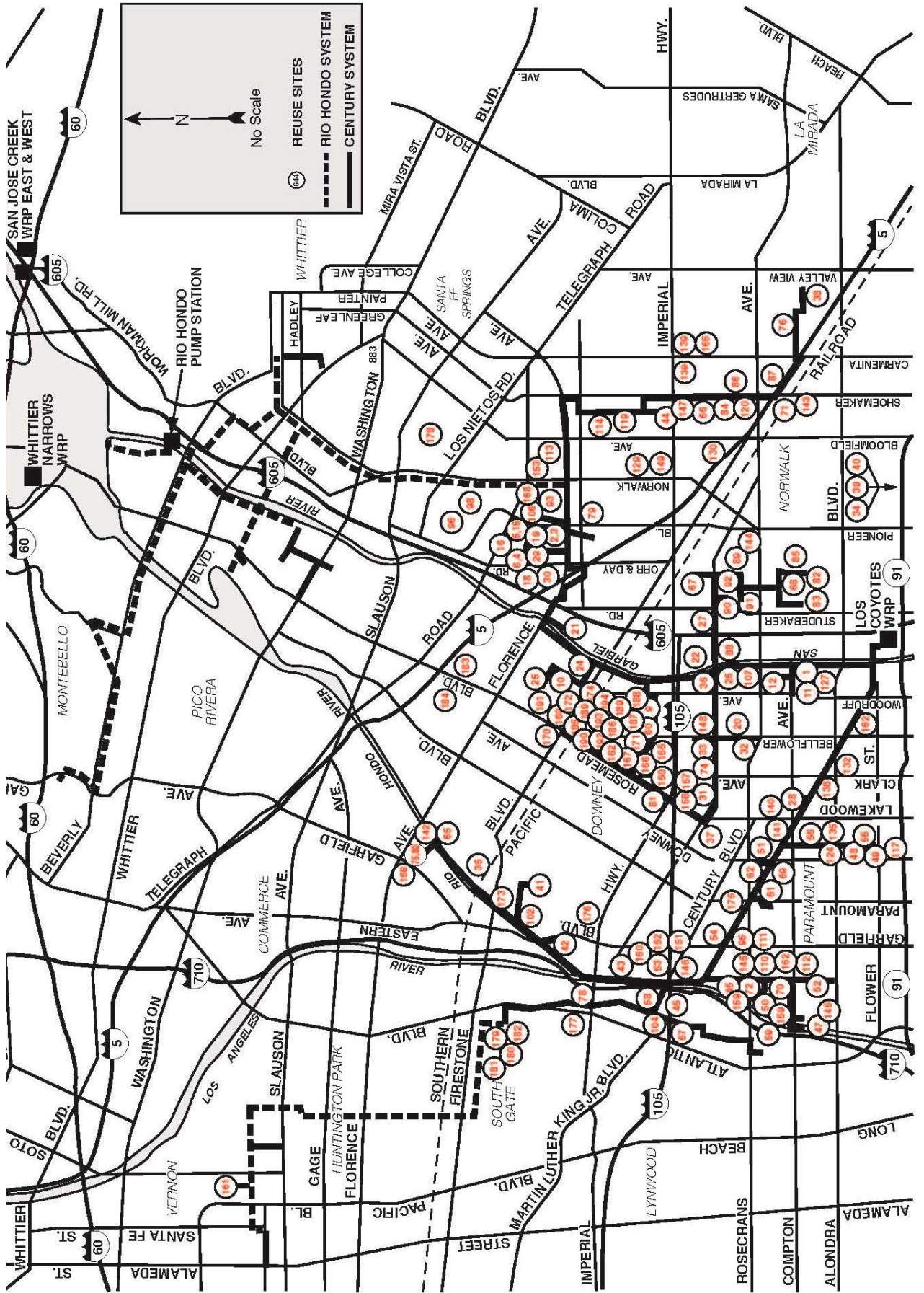
FIGURE 10 CENTRAL BASIN MUNICIPAL WATER DISTRICT RECYCLED WATER DISTRIBUTION SYSTEM
