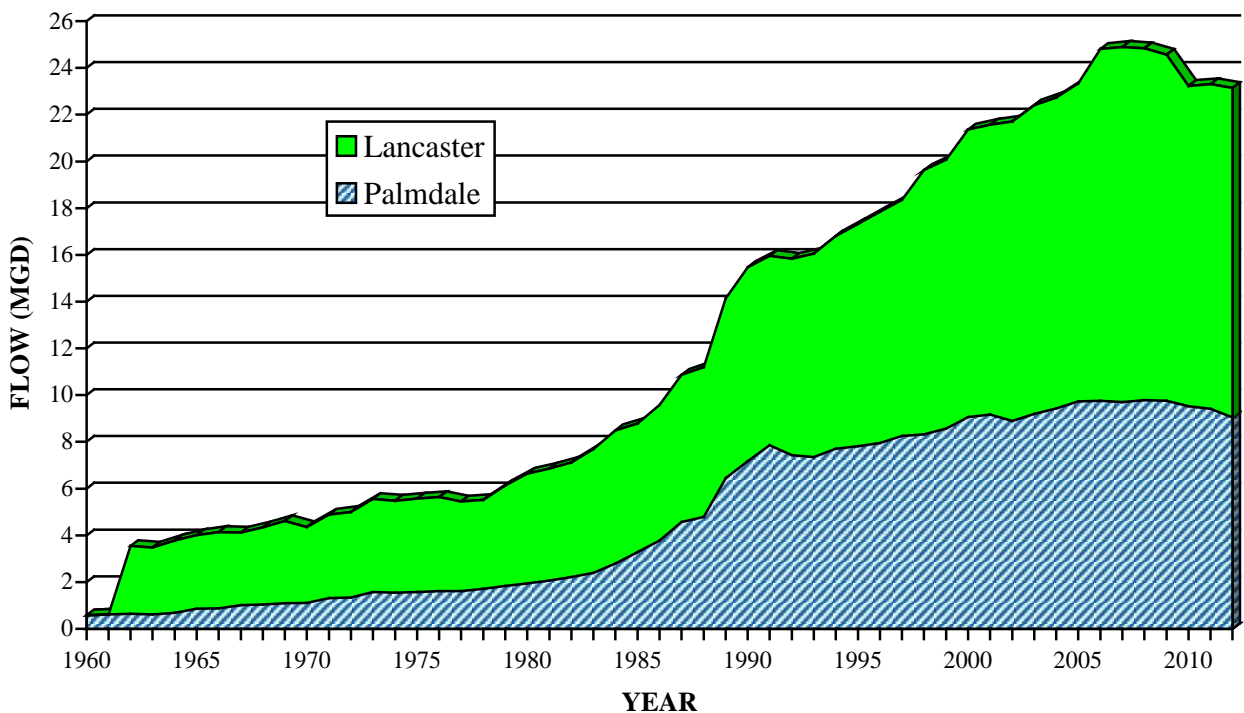
FIGURE 17 ANTELOPE VALLEY WRPs INFLUENT FLOW 1960-2013
