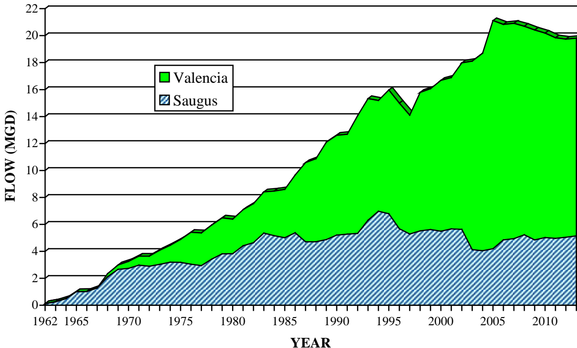
FIGURE 15 SANTA CLARITA VALLEY JOINT SEWERAGE SYSTEM RECYCLED WATER PRODUCTION 1962-2013
