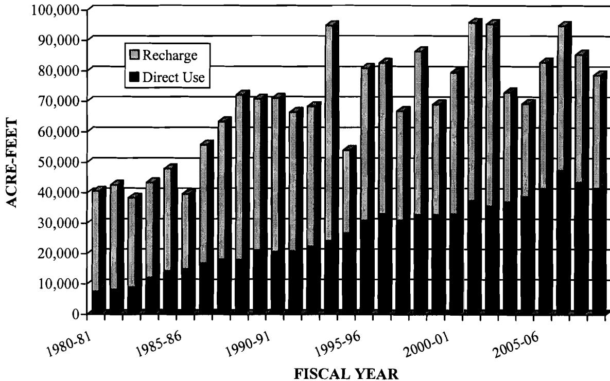
FIGURE 3 DIRECT NONPOTABLE REUSE VS. GROUNDWATER RECHARGE 1980-81 TO 2008-09
