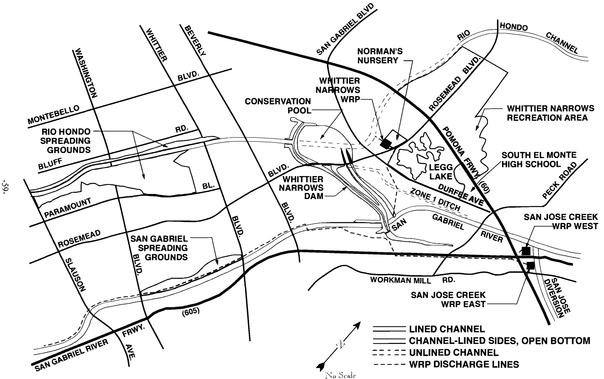
FIGURE 14 WHITTIER NARROWS WRP REUSE SITES
