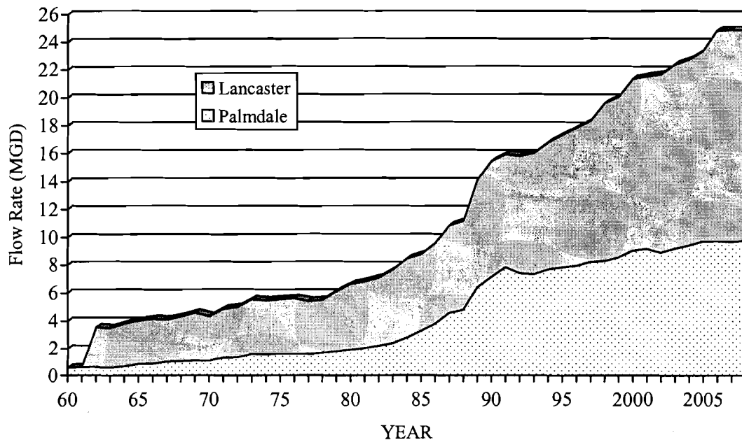
FIGURE 17 ANTELOPE VALLEY WRPs INFLUENT FLOW 1960-2008
