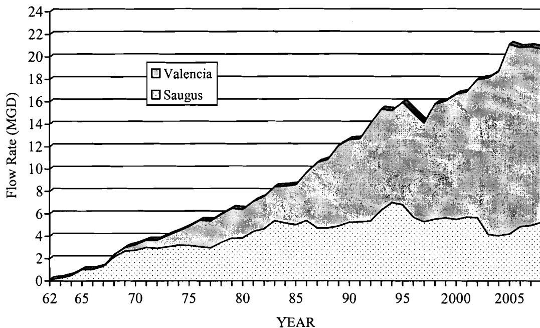
FIGURE 15 SANTA CLARITA VALLEY JOINT SEWERAGE SYSTEM RECYCLED WATER PRODUCTION 1962-2008
