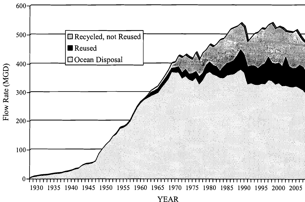
FIGURE 2 SANITATION DISTRICTS' FLOW DIVERSION TO RECYCLING 1928-2008
