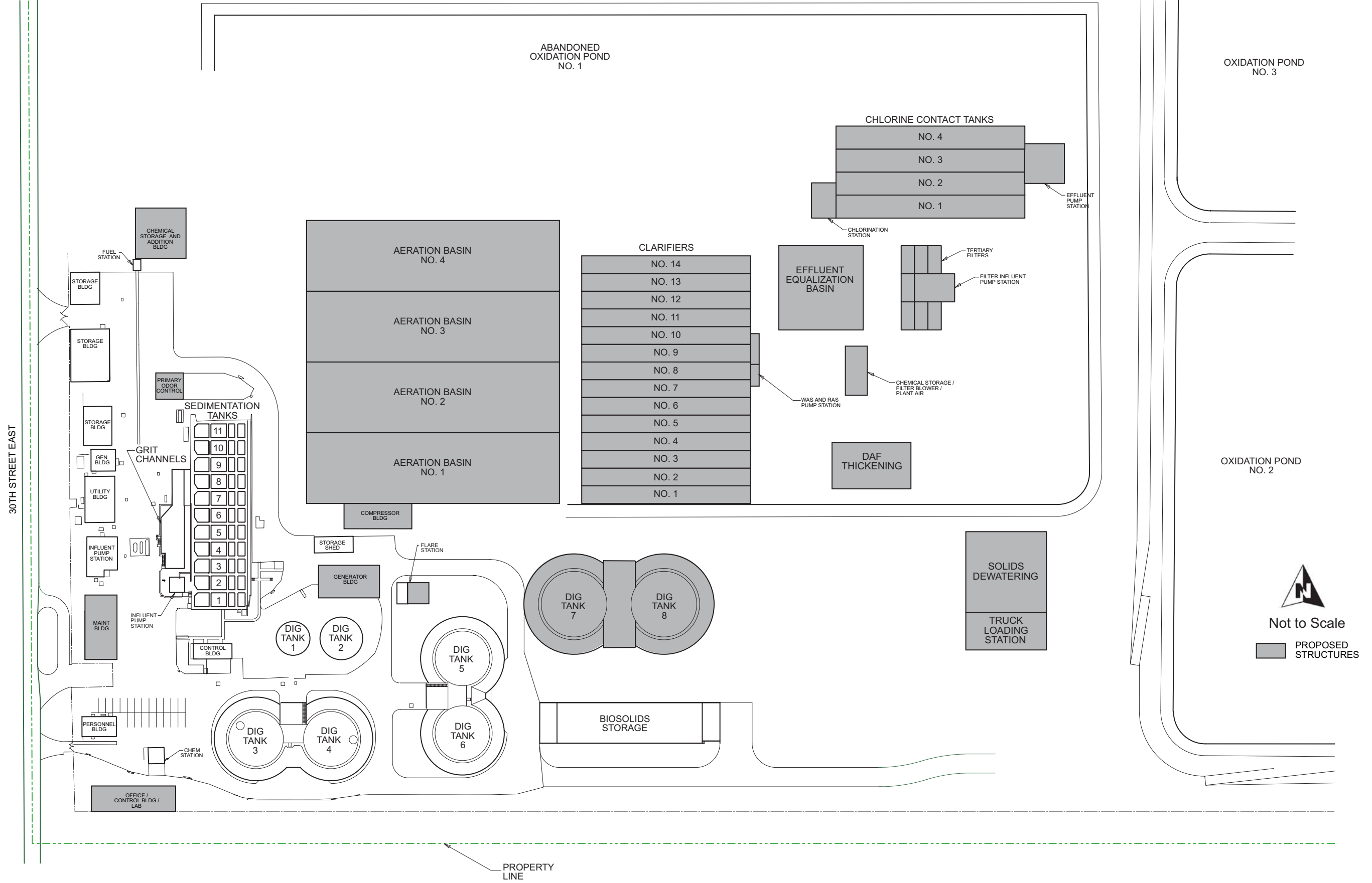
Figure ES-7 Palmdale Water Reclamation Plant Stage V
