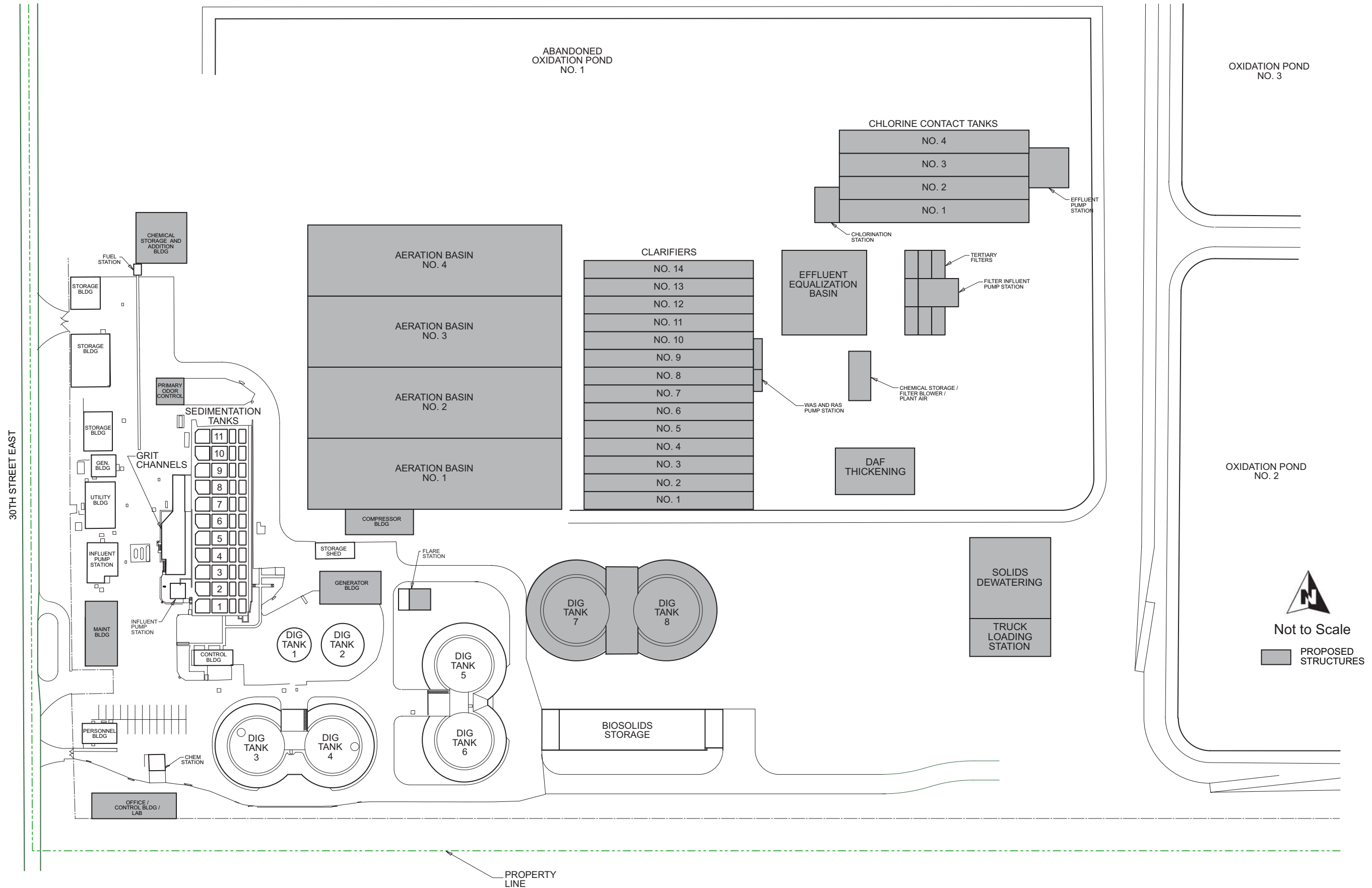
Figure 7-2 Palmdale Water Reclamation Plant Stage V
