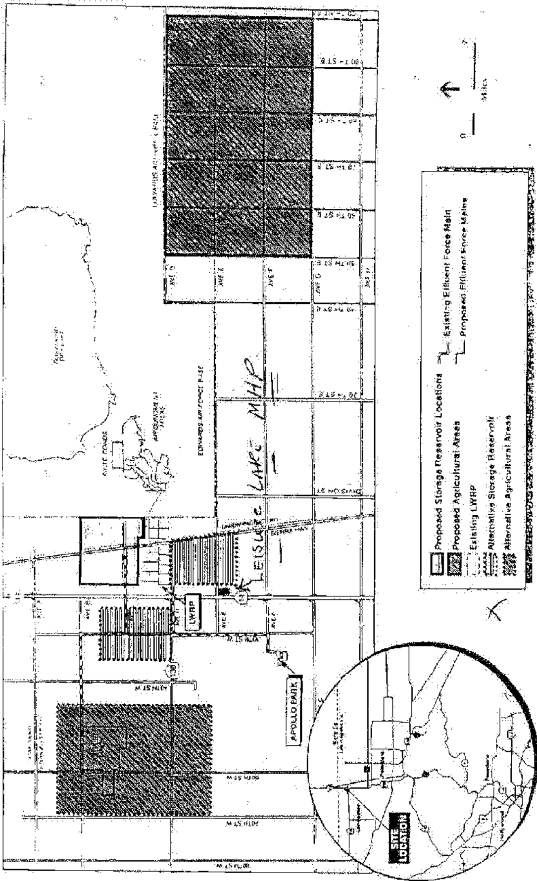
Figure 1 Potential Floodplain of EWRP 7029 Plus Storage Reservoir and Agricultural Land
